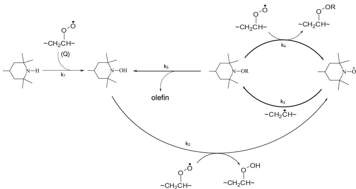
Kinetics of Radical Scavenging Reactions by HALS
